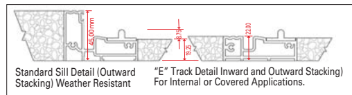
SILL DETAILS: Origin E Track used for level floor option.
